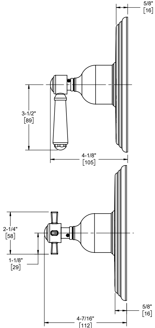
(TO-PB2L-34 SHOWN)
